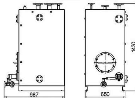
Diesel Oil Tank 600
