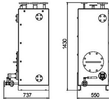
Diesel Oil Tank 300
